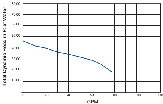
Performance Curve Marathon Motor 7.0 Amp Feet of Water/GPM
