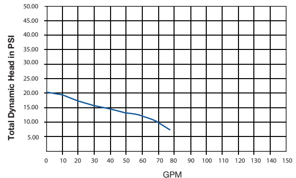
Performance Curve Marathon Motor 7.0 Amp PSI/GPM
